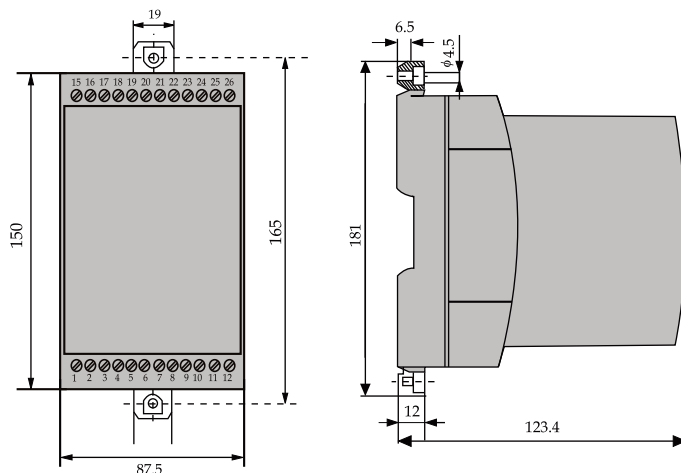
Fig. 7. Theta Series in housing T24, screw hole mounting brackets pulled out.
