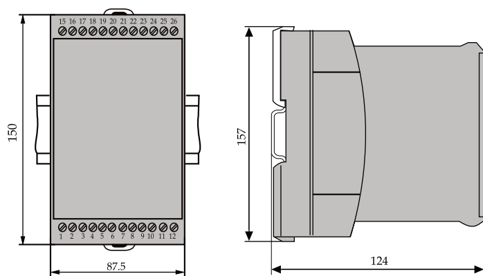
Fig. 6. Theta Series in housing T24 clipped onto a top-hat rail (35 X 15 mm or 35 X 7.5 mm, acc. to EN 50 022).
